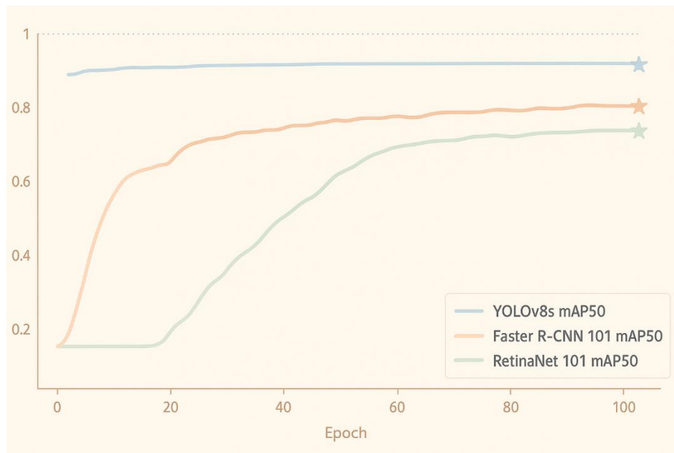
Figura 2. Mean Average Precision (mAP 50 )
